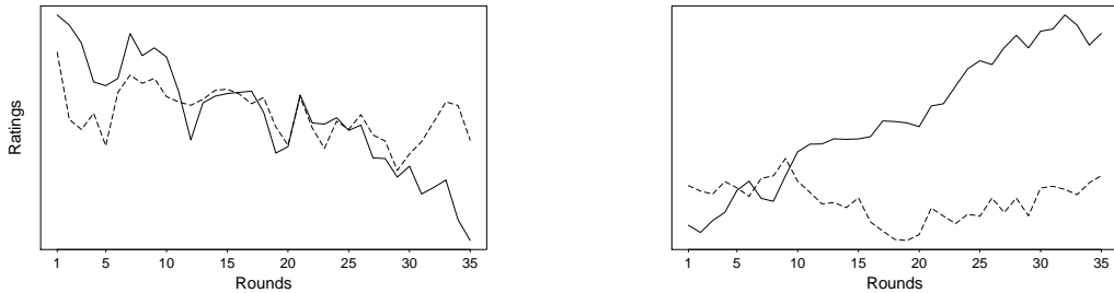
Figure 4: Difference in simulation for the correlated (left) and uncorrelated (right) attacking and defensive ratings for a single team throughout a 35-rounds season.
